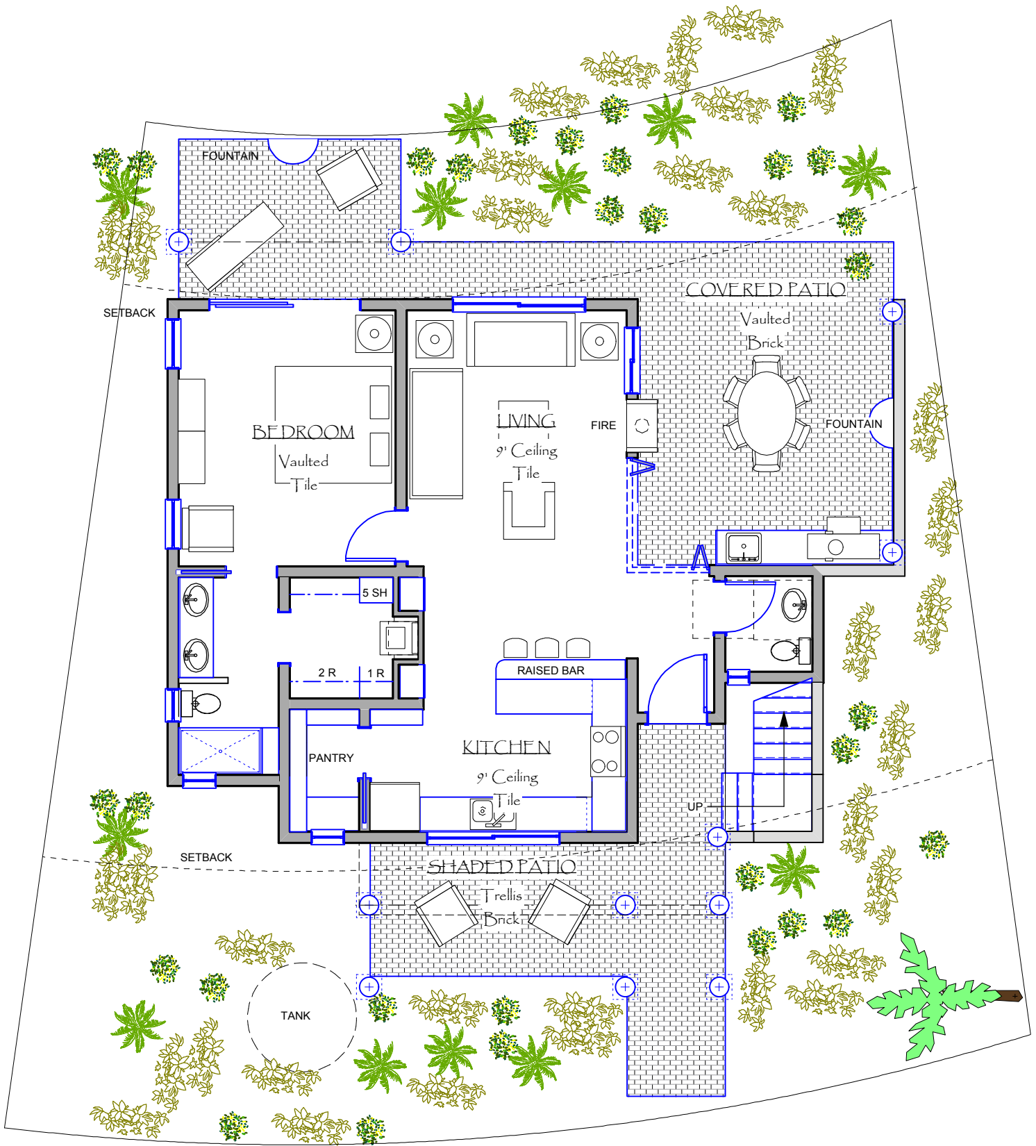
1 MAIN FLOOR PLAN C1 Scale: 1/8" = 1'-0"
