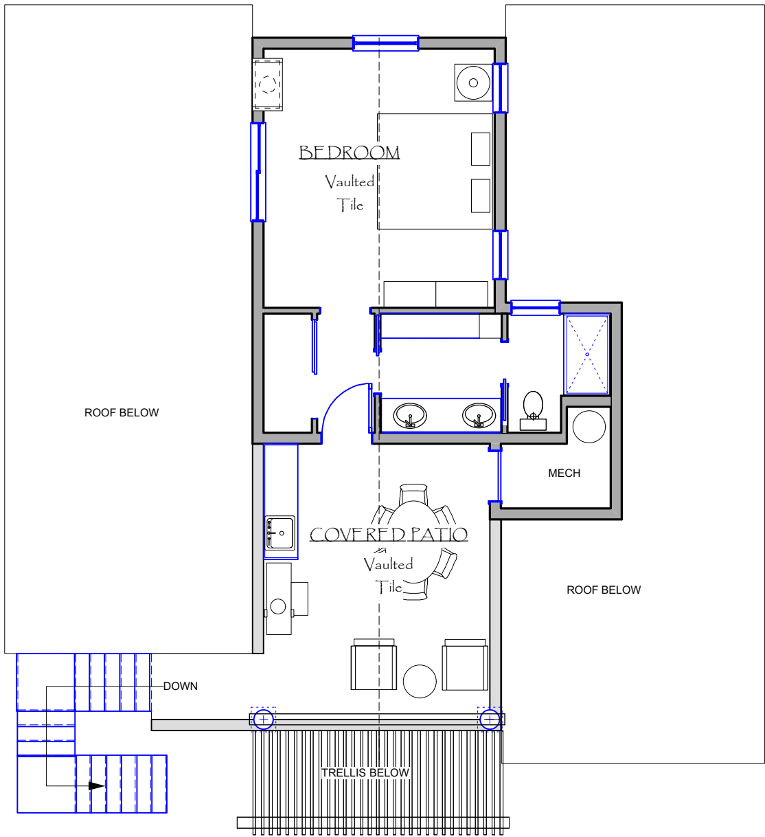
2 B2 UPPER FLOOR PLAN Scale: 1/8" = 1'-0"
